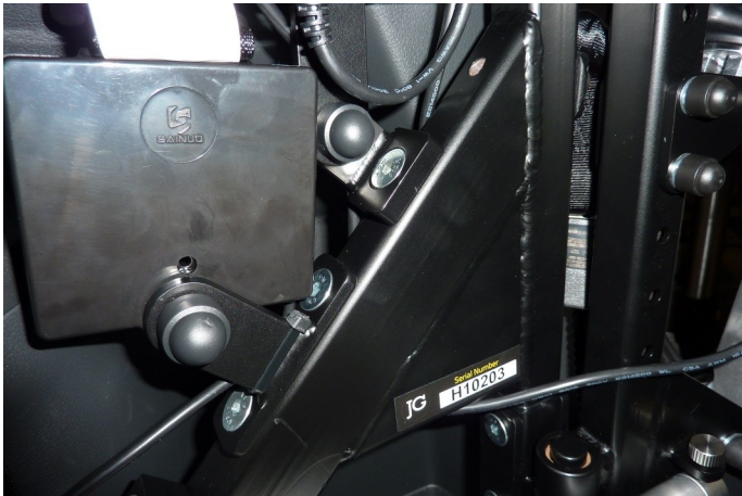
Fit the restraint reel and buckle and the control box in suitable positions.
