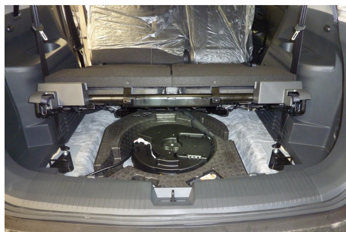
Remove the sub-floor cover and tilt the 6th and 7th seats up by pulling the two release belts.
